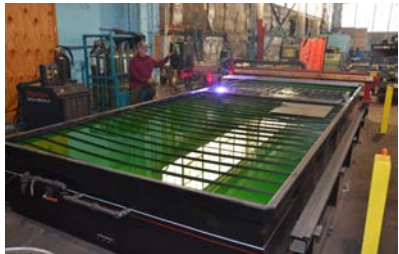
96" x 240" plasma – 1.5" A36
