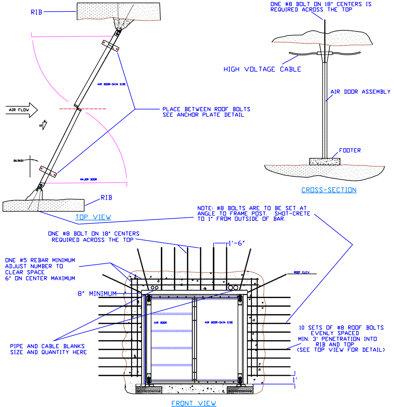
AIR DOOR CONSTRUCTION - Roof and Rib Anchor Details
